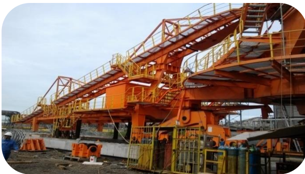
BOOM & BELT CONVEYOR
